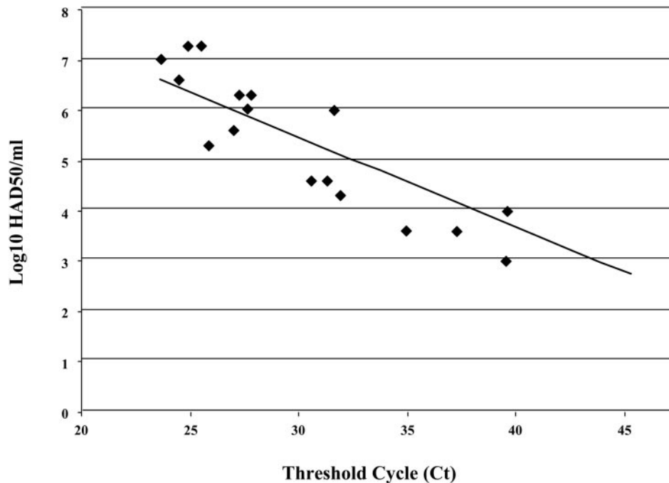
FIG. 1. Sensitivity of the ASFV real-time PCR assay was calculated by using ASFV samples obtained from infected cell culture supernatants or blood samples from infected pigs. An inverse linear relationship ( r = 0.9237 ) exists between cycle threshold and the logarithm of HAD 50 per milliliter present in the sample.
